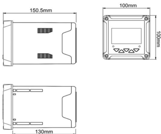
Fig.1 Product dimensions (Unit: mm)
