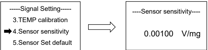
Fig.54 Sensor sensitivity
