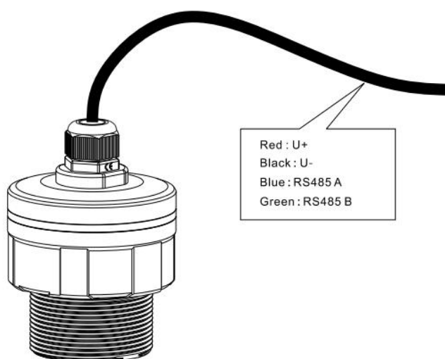
Figure1 Diagram of 2-wire version
