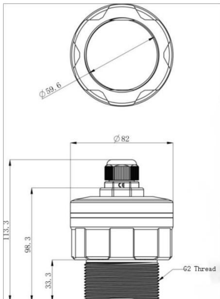
Figure3 Dimensions (unit: mm)
